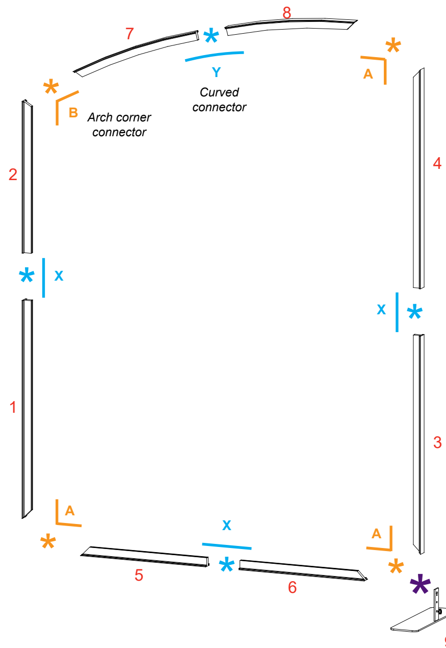
FRONT VIEW
